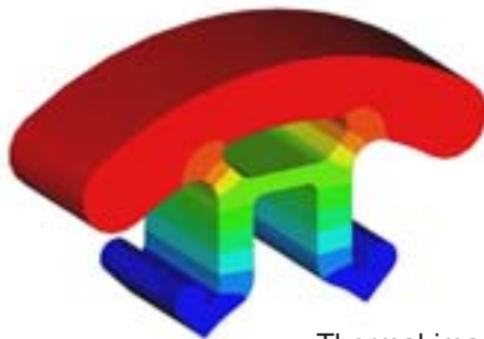
Thermal image of clutch shoe
