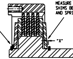
SHIM DETAIL "A"
