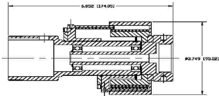
Bottle Capping Clutch - HSV 4.5 (4.5 Nm/40 lbin)
