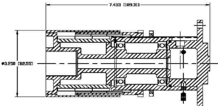
Bottle Capping Clutch - HSV 9 (9 Nm/80 lbin)
