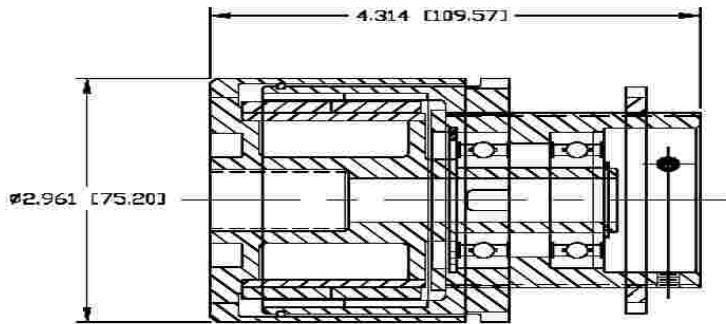
Bottle Capping Clutch - HSV 3 (3Nm/26-27 lbin)
