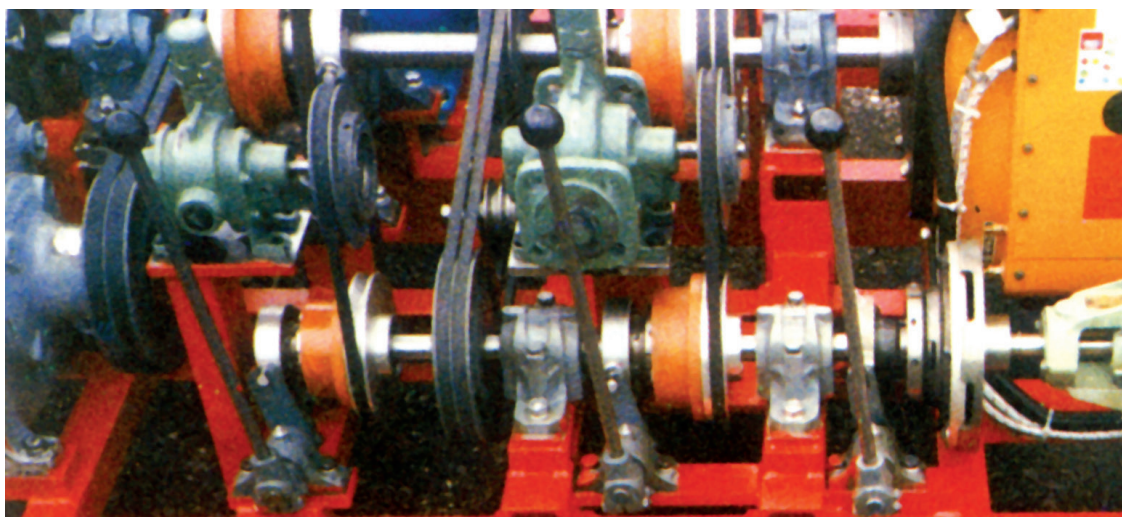
Conax® clutches, type CM in a combined transmission set for bunker boats, inclusively Planox® clutches.
