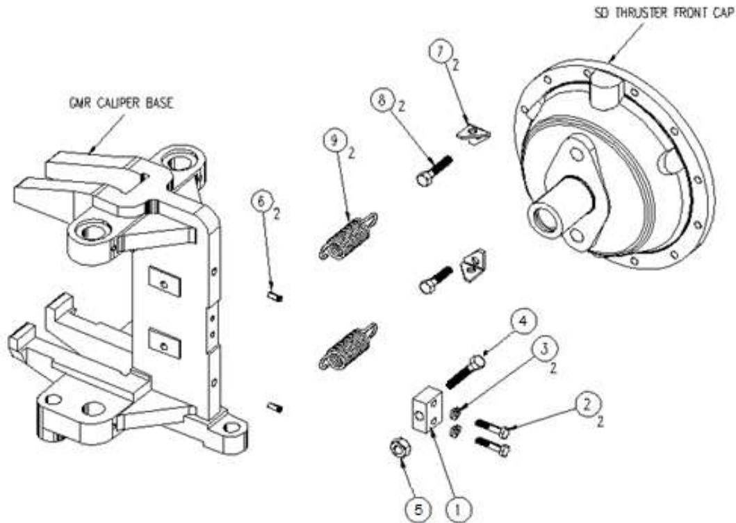
FIGURE 4 – Inclined Mounting Kit
