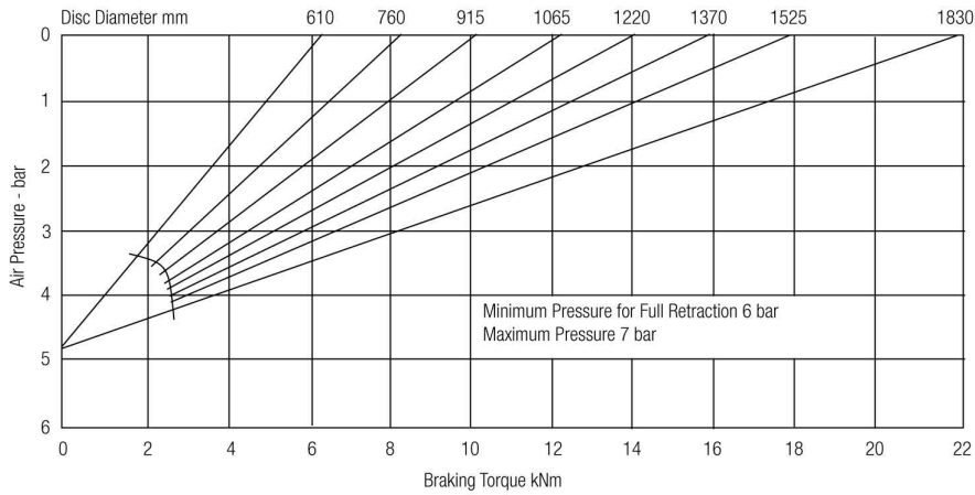
Brake performance at 25 kN braking force
