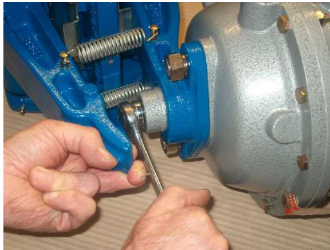
FIGURE 5 – Thruster Setting
