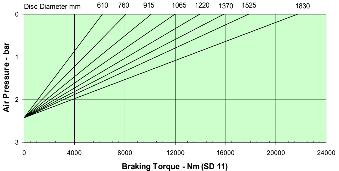
Braking Performance at 25 kN Braking Force
