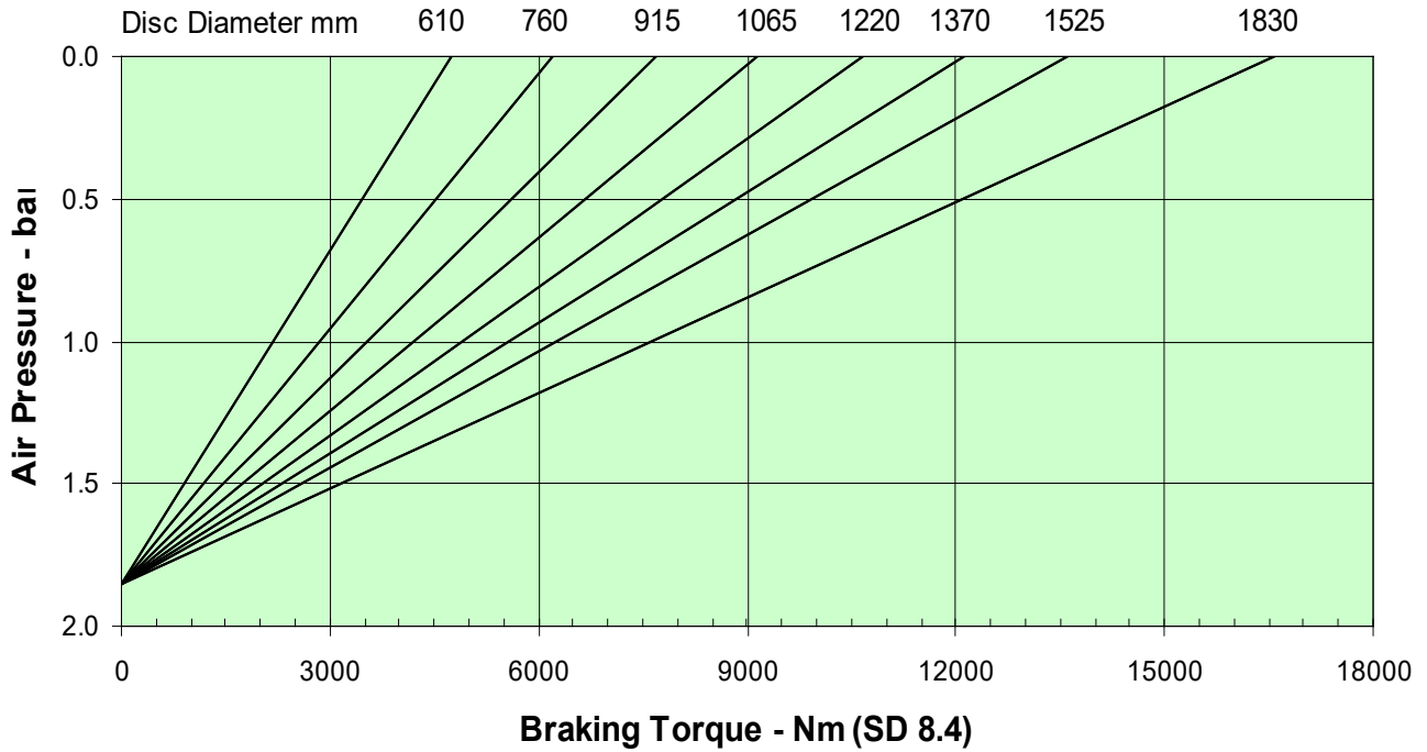
Braking Performance at 19.5 kN Braking Force
