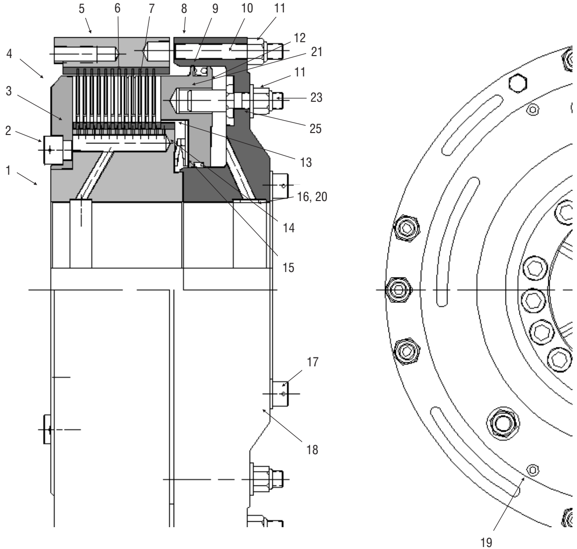
Component Parts
