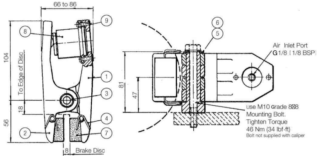
Disc Brake Caliper Assembly Type MUP Complete assembly (Caliper and thruster) Part No. 678919
