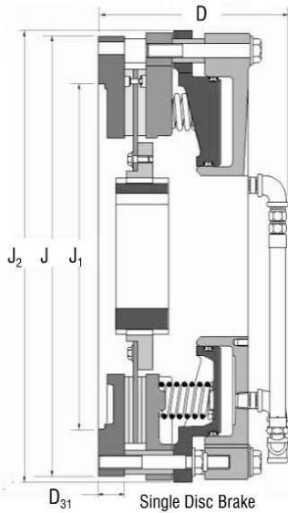
Single Disc Brake
